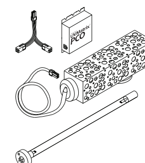
The UVMatrix™ PCO-24-10 features a PCO module and an EZ-Light 6P Germicidal UV-C lamp (UV lamp available in 12" and 17" lengths, and uses the Quick connect Y adapter to connect .
