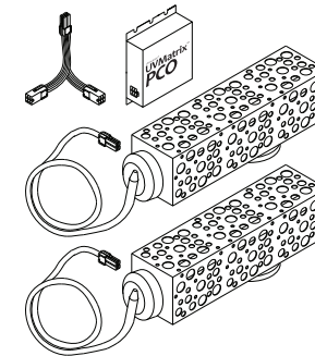
The UVMatrix™ PCO-24-2-10 features two 10" PCO modules that connect to the power supply using a Quick Connect Y Adapter.
